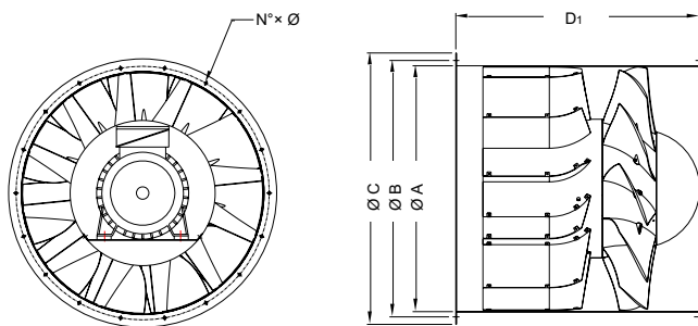
Direct Driven
