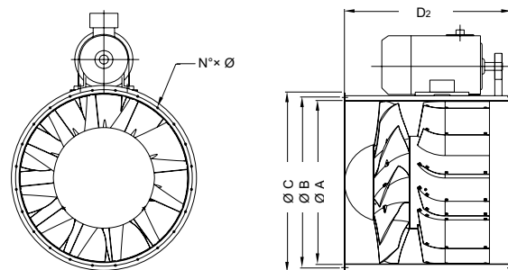
Belt Driven
